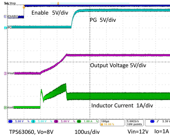
Figure 33. Startup After Enable
