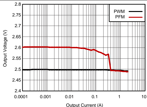
Figure 21. Output Voltage vs Output Current
