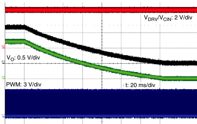
Power Off with V_{IN} ramping down V_{IN} = 12\text{ V} , V_{OUT} = 1.2\text{ V} , F_S = 500\text{ kHz}
