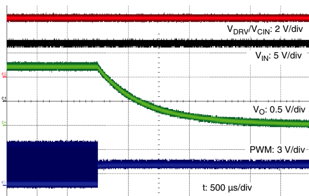
PWM Turn-off with V_{IN} = 12\text{ V} , V_{OUT} = 1.2\text{ V} , F_S = 500\text{ kHz}
