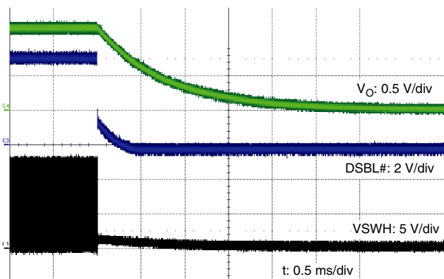
Disable with V_{IN} = 12\text{ V} , V_{OUT} = 1.2\text{ V} , F_S = 500\text{ kHz}
