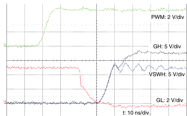
Switching Waveforms at PWM rising edge V_{IN} = 12\text{ V} , V_{OUT} = 1.2\text{ V} , F_S = 500\text{ kHz} , I_{OUT} = 0\text{ A}
