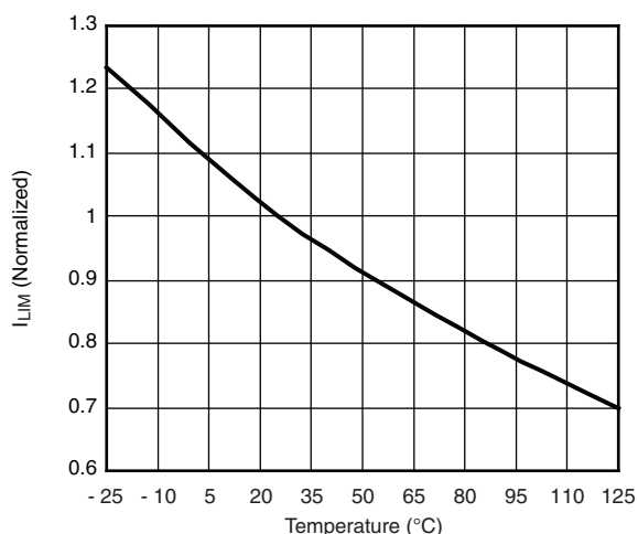
Peak Current Limit vs. Temperature (Normalized)
