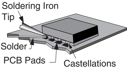
Figure 34: Soldering Technique
