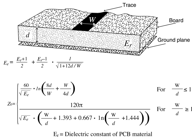
Figure 32: Microstrip Formulas
