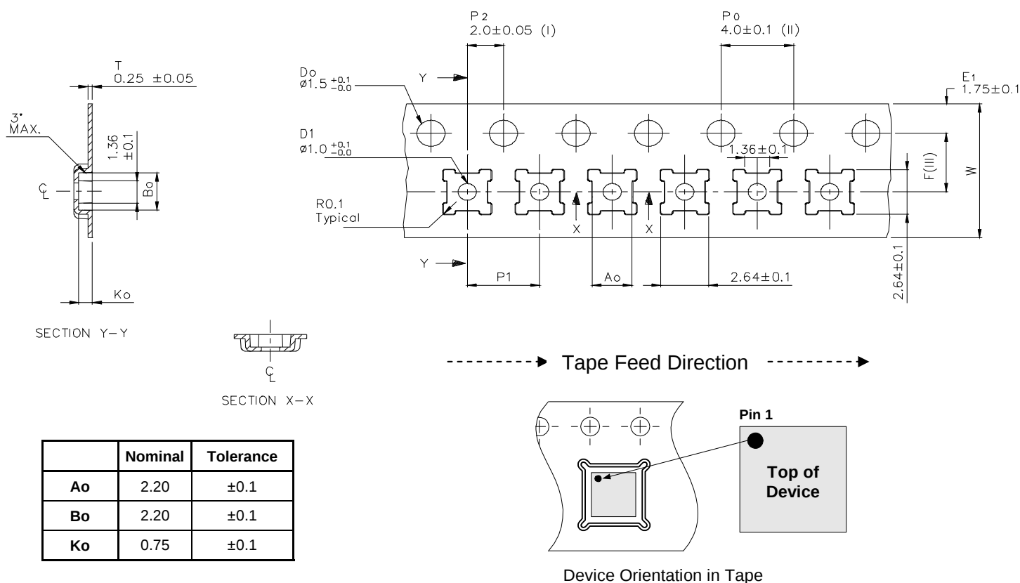
Figure 33. Tape and Reel Specifications 12-lead 2 × 2 × 0.55 mm QFN
