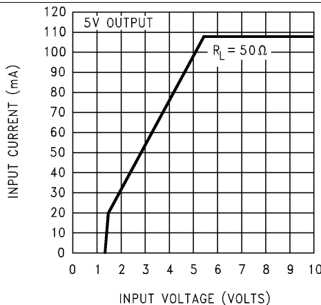
Figure 4. Input Current
