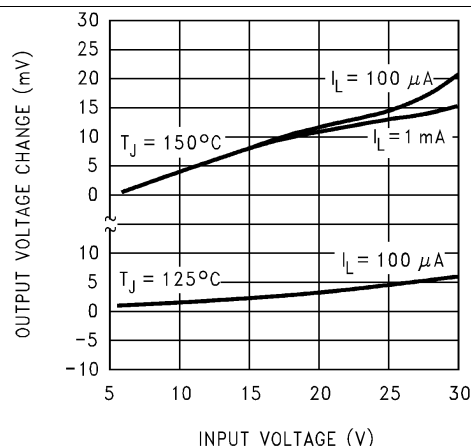
Figure 26. Line Regulation
