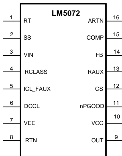
Figure 1. 16 Lead TSSOP-EP
