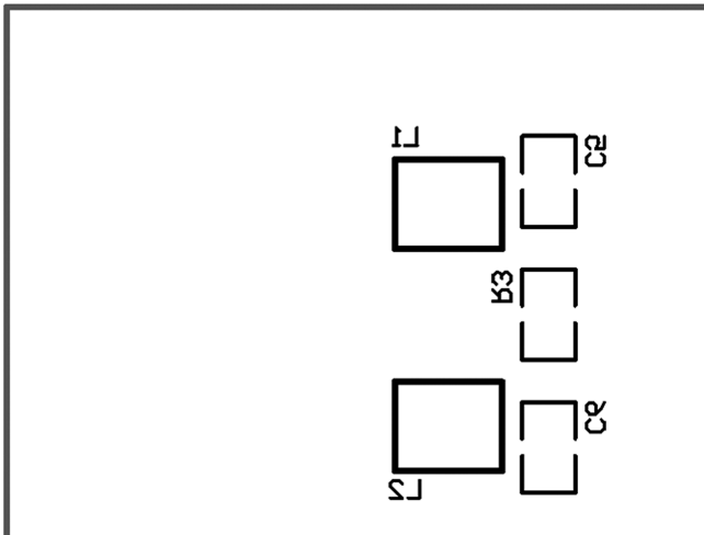
Bottom Silkscreen
