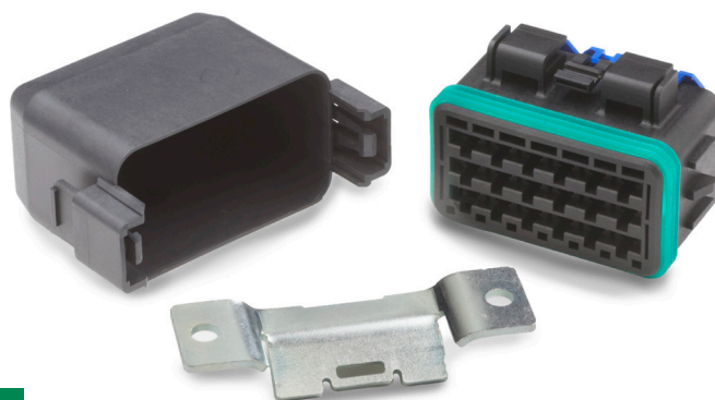
HWB18 accepts plug-in circuit protection components with 280 style footprint.
