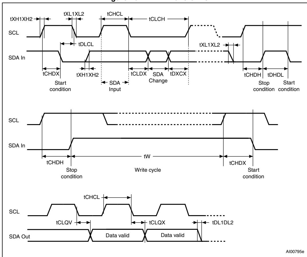
Figure 16. I 2 C AC waveforms
