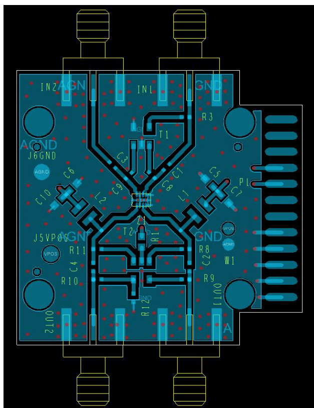
Figure 26. Evaluation Board Layout, Top Layer
