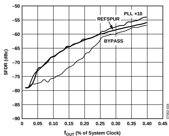
Figure 13. SFDR Without the Internal PLL (REF_CLK = 25 MHz \times 10 = 250 MHz Using PLL, 4 mA DAC Full-Scale Current)
