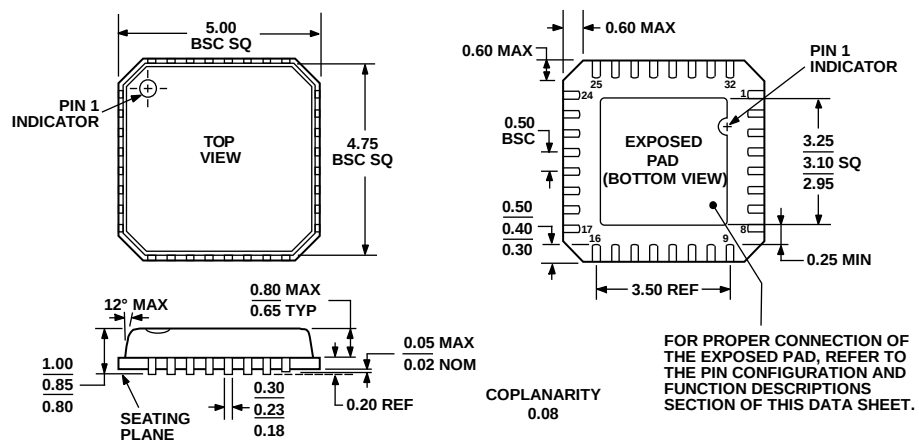
Figure 36. 32-Lead Frame Chip Scale Package [LFCSP_VQ] 5 mm x 5 mm Body, Very Thin Quad (CP-32-2) Dimensions shown in millimeters
