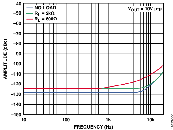
Figure 57. Third Harmonic Distortion vs. Frequency ( G = 1 )
