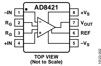
Figure 3. Pin Configuration
