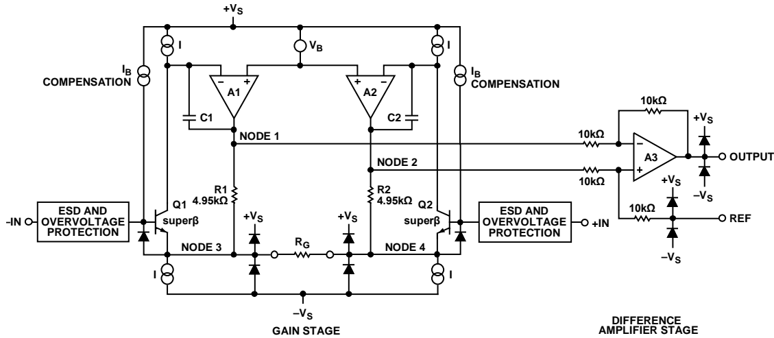
Figure 61. Simplified Schematic
