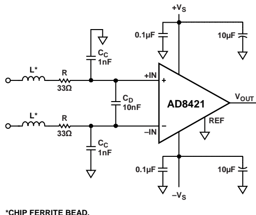
Figure 68. RFI Suppression
