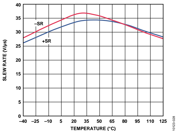
Figure 30. Slew Rate vs. Temperature, V_S = \pm 15 V ( G = 1 )
