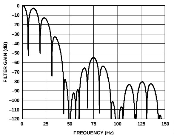
Figure 44. Sinc^4 Filter Response (FS[9:0] = 96, Chop Enabled, REJ60 = 1)
